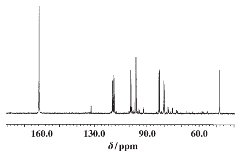
Figure 2. 31 P-{ 1 H} NMR spectrum obtained after 18 h of reflux of Na 2 Se and PhPCl 2 in toluene.
