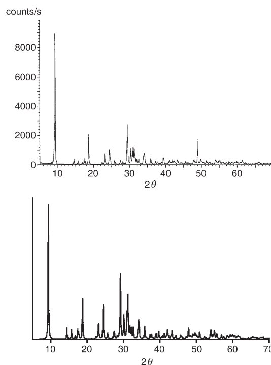
Figure 1. The upper spectrum shows the actual powder diffraction pattern obtained for 1 ; the lower spectrum shows the powder diffraction pattern simulated from single crystal data of 1 .
