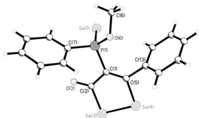
Figure 5. The X-ray structure of 9 . Selected bond lengths [Å] and angles [°] (esd's in parentheses). Se(1)–P(1) 2.096(3), P(1)–O(6) 1.591(7), C(2)–Se(3) 1.948(10), Se(3)–Se(4) 2.3082(16), Se(4)–C(5) 1.895(10), O(6)–C(6) 1.469(13), C(2)–O(2) 1.202(12); C(1)–P(1)–Se(1) 113.1(3), C(5)–C(1)–P(1) 126.6(8), C(2)–C(1)–P(1) 112.9(7), C(2)–C(1)–P(1) 112.9(7), O(2)–C(2)–C(1) 126.4(9), O(2)–C(2)–Se(3) 119.7(8), C(1)–C(2)–Se(3) 113.9(7), C(2)–Se(3)–Se(4) 92.4(3), C(5)–Se(4)–Se(3) 91.1(3), C(1)–C(5)–Se(4) 122.0(8), C(5)–C(1)–C(2) 120.3(9).
