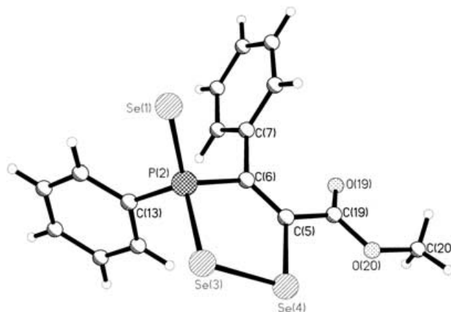
Figure 4. The X-ray structure of 8 . Selected bond lengths [Å] and angles [°] (esd's in parentheses): Se(1)–P(2) 2.096(2), P(2)–Se(3) 2.2387(19), Se(3)–Se(4) 2.3286(11), Se(4)–C(5) 1.924(6), C(5)–C(6) 1.323(9); Se(1)–P(2)–Se(3) 112.21(9), P(2)–Se(3)–Se(4) 94.78(5), C(5)–Se(4)–Se(3) 96.1(2), C(5)–C(6)–P(2) 112.3(4), C(6)–C(5)–Se(4) 123.8(5).
